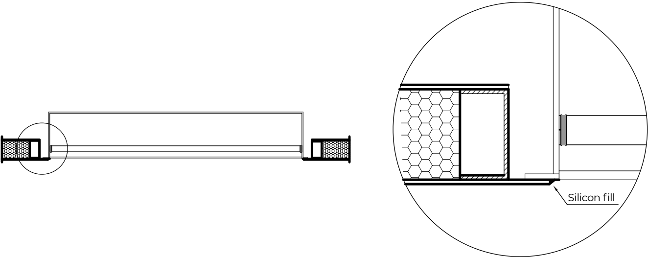
Connecting detail between ceiling panel and light
